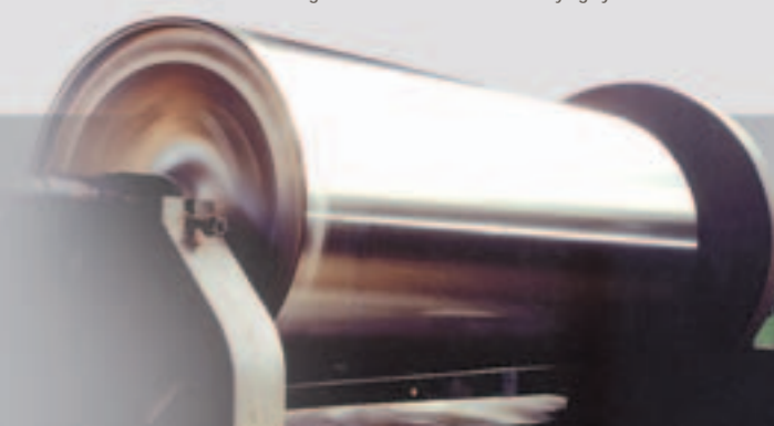
Rectification d'un cylindre sécheur - Ø1500mmx3000mm Grinding of a Ø1500mm x 3000mm drying cylinder
